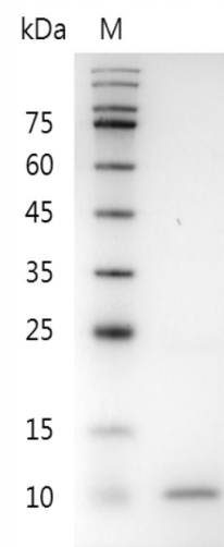
SDS-PAGE analysis of recombinant mouse BMP-4
